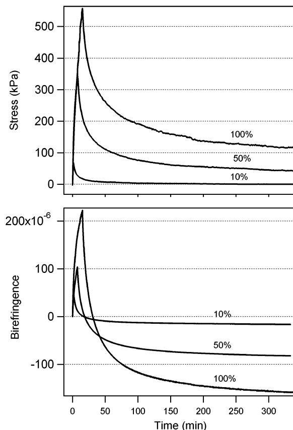
Figure 1. Simultaneous tensile stress and birefringence of ES at various strains. Specimens were elongated at 1 mm/min and held under strain after reaching the specified strain.
