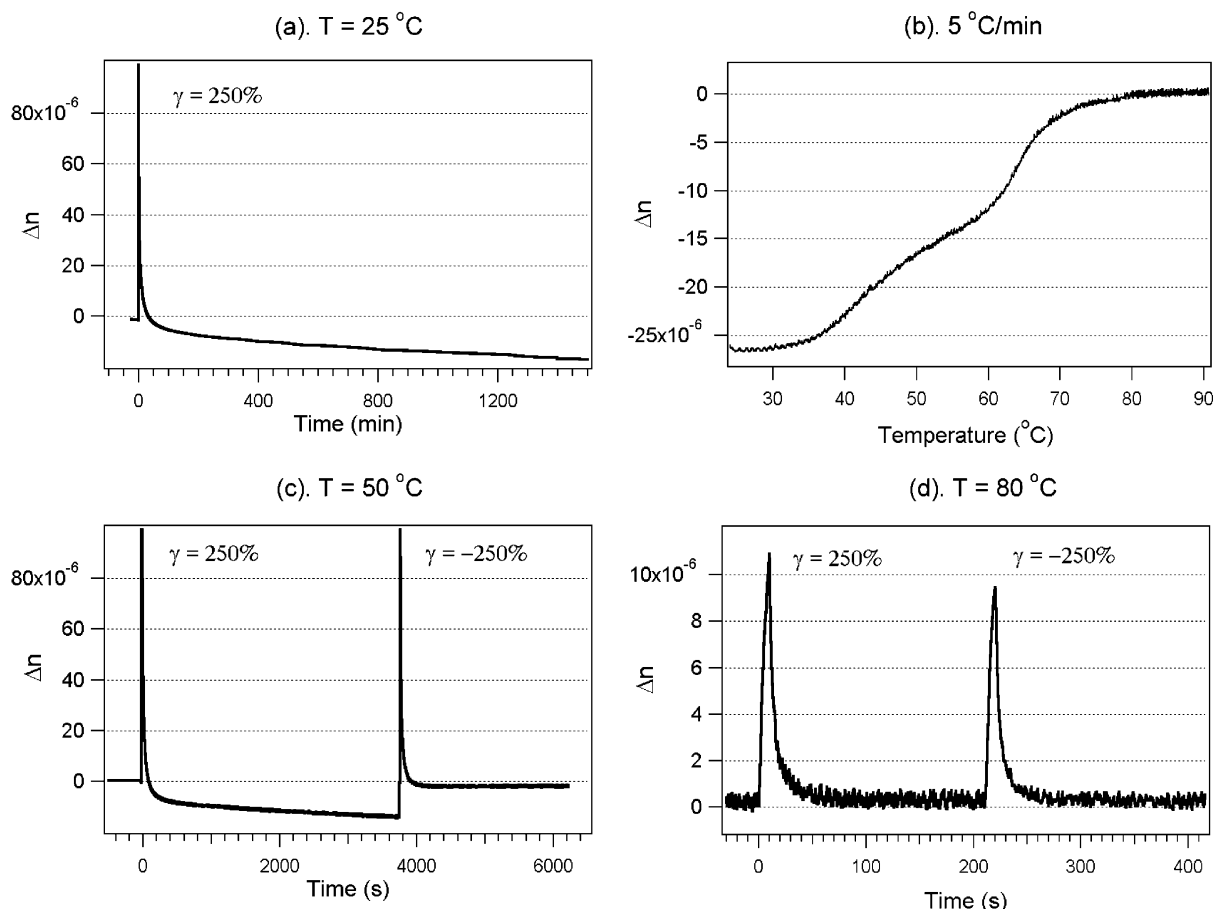
Figure 5. Birefringence response of ES under step-shear deformations: (a) step-shear at 25 °C; (b) under 250% strain from part (a), heat at 5 °C/min; (c) reverse step-shear at 50 °C; and (d) reverse step-shear at 80 °C.
