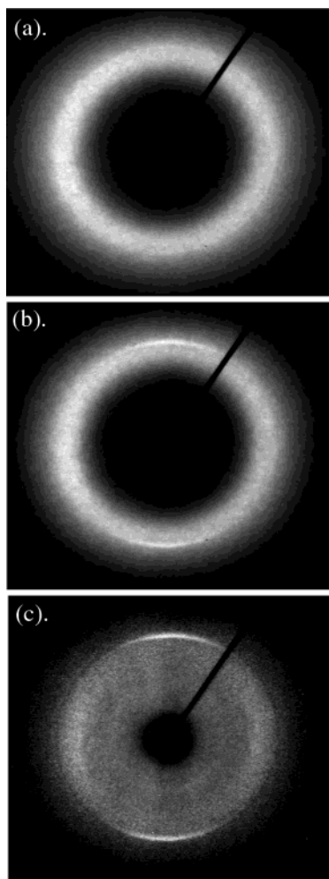
Figure 6. 2-D WAXS patterns of ES with strain axis along the vertical direction: (a) unstretched, (b) at 300% strain, and (c) at 300% strain after subtraction of the unstretched scattering pattern.
