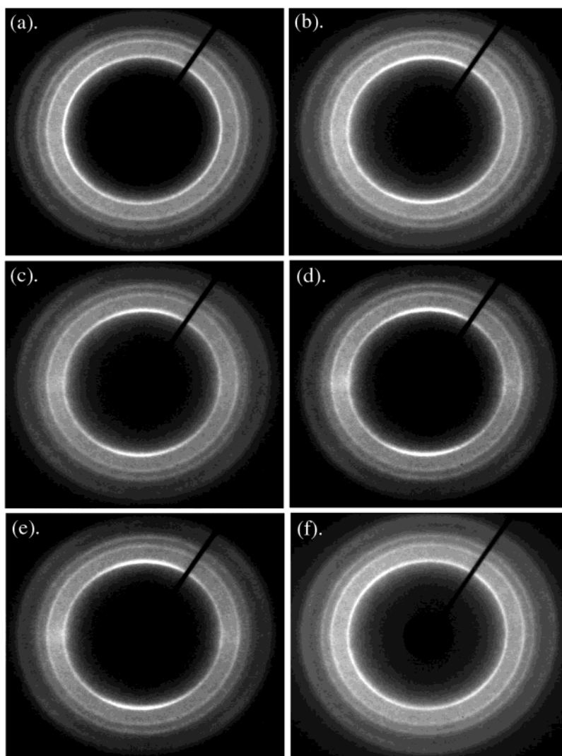
Figure 8. 2-D WAXS patterns of the ES/PI blend: (a) unstretched, (b) at 100% strain, (c) at 200%, (d) at 300%, (e) at 300% after 1 h relaxation, and (f) after 1 day free of 300% strain for 1 h.
