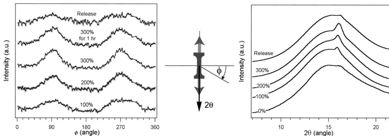
Figure 7. 1-D scattering profiles of ES at various strains: (a) azimuthal intensity plots integrated through an annulus of the meridional arcs; (b) intensity profiles along the meridional axis. Curves have been shifted along the y -axis for clarity.
