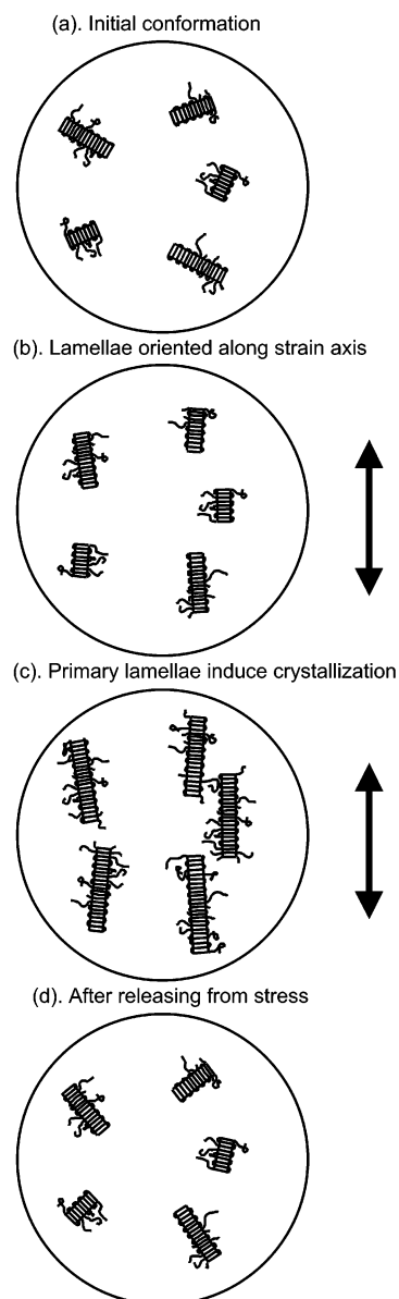
Figure 11. Schematic of a lamellae orientation and growth model of ES: (a) before deformation, lamellae are oriented isotropically; (b) deformation orients the lamellae along the strain axis; (c) oriented lamellae induce subsequent crystallization; and (d) when release from strain, the oriented lamellae are able to relax.
