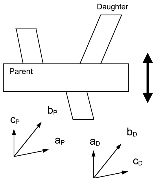
Figure 12. Schematic of a daughter lamellae growth model of ES in blends containing crystallites of the \alpha -form.
