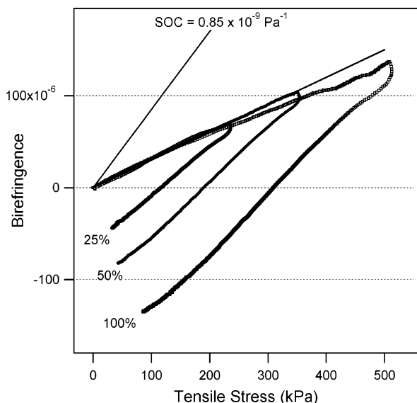
Figure 3. Simultaneous tensile stress and birefringence response of ES presented in the form of birefringence–stress curves. The upward curves show the stretching response while the downward curves correspond to 6 h stress relaxation.
