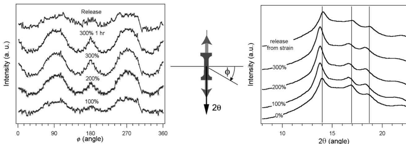
Figure 9. 1-D WAXS profiles of the ES/PI blend in tensile stretching at various strains: (a) azimuthal intensity plots of the (110) scattering peak; (b) intensity profiles along the meridional axis. Curves have been shifted vertically for clarity.
