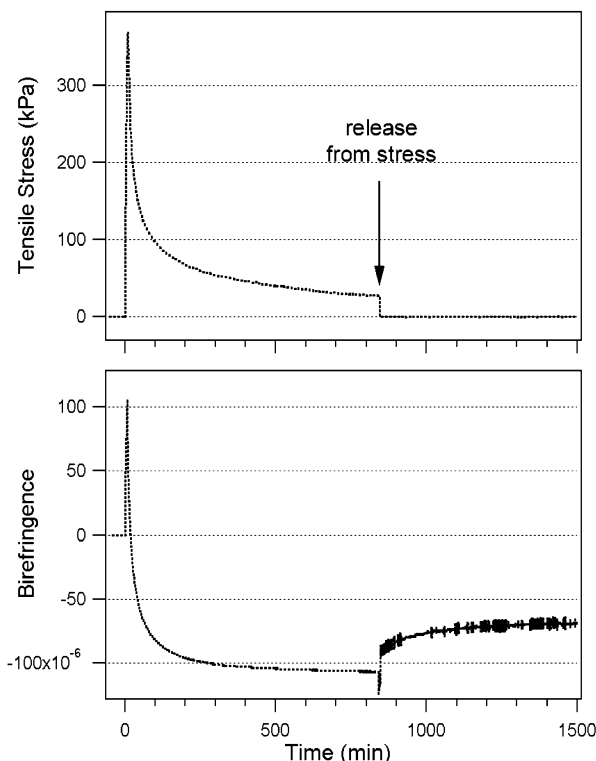
Figure 4. Residual birefringence of ES subjected to tensile stretching. Sample was initially subjected to 50% strain and held for 14 h to follow the relaxation dynamics. The sample was then free from strain, and the residual birefringence was monitored.
