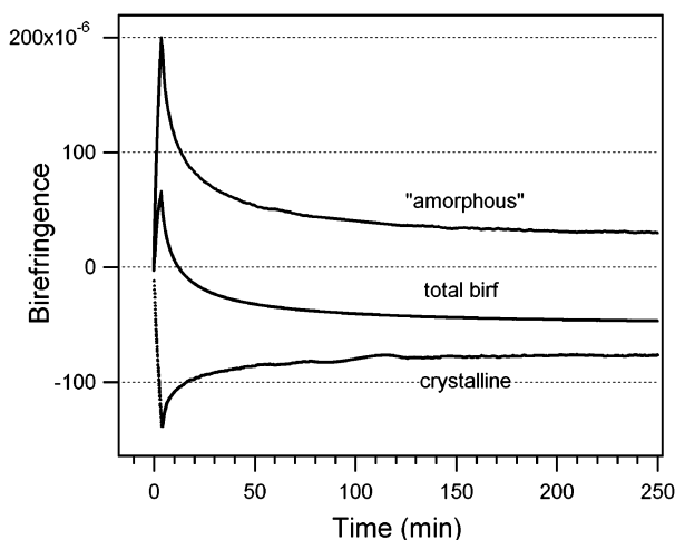
Figure 10. Crystalline and amorphous contributions of the birefringence of ES subjected to 25% step-shear deformation.
